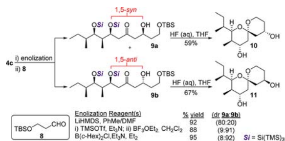
Scheme 3. 1,5-Directed Aldol Reaction of 4c
