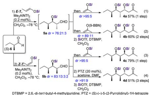
Scheme 3. 1,5-Directed Aldol Reaction of 4c
